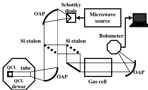
Fig. 4. Setup used for gas spectroscopy experiments.
