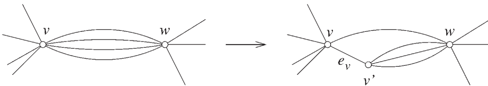
FIGURE 2. Extruding an edge from v .
