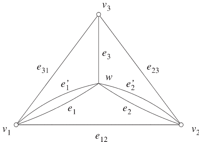
FIGURE 3. The edge labels of K_4'' .
