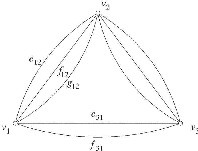
FIGURE 1. C_3(3, 3, 2) for Example 2.2 and Proposition 6.10.
