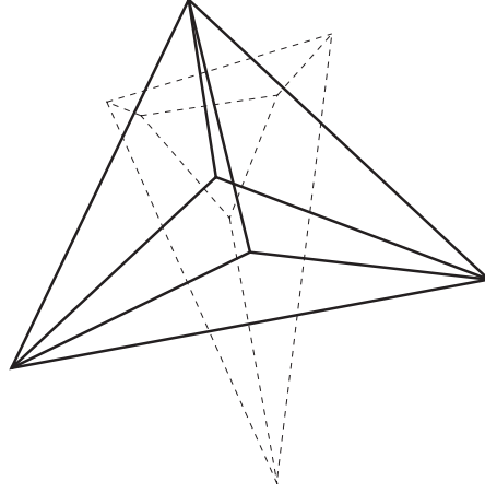
FIGURE 3. Reciprocal for a 2-sphere in \mathbb{R}^2 .
