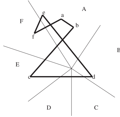
FIGURE 5. Non-convex reciprocal.
