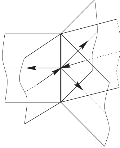
FIGURE 1. Equilibrium of forces at 1-cell.
