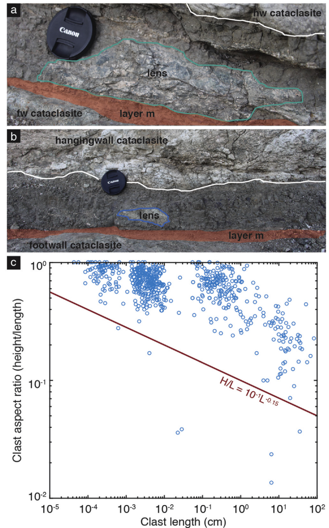
Fig. 5. Lenticular clasts in the inner fault core. a: Photograph showing an example of a lenticular clast from footwall outer fault-core material in the inner fault core. b: An example from the hangingwall outer fault core in the inner fault core. c: Clast aspect ratios plotted against clast maximum length for clasts from SEM images, photomicrographs, field photographs, and field measurements.
