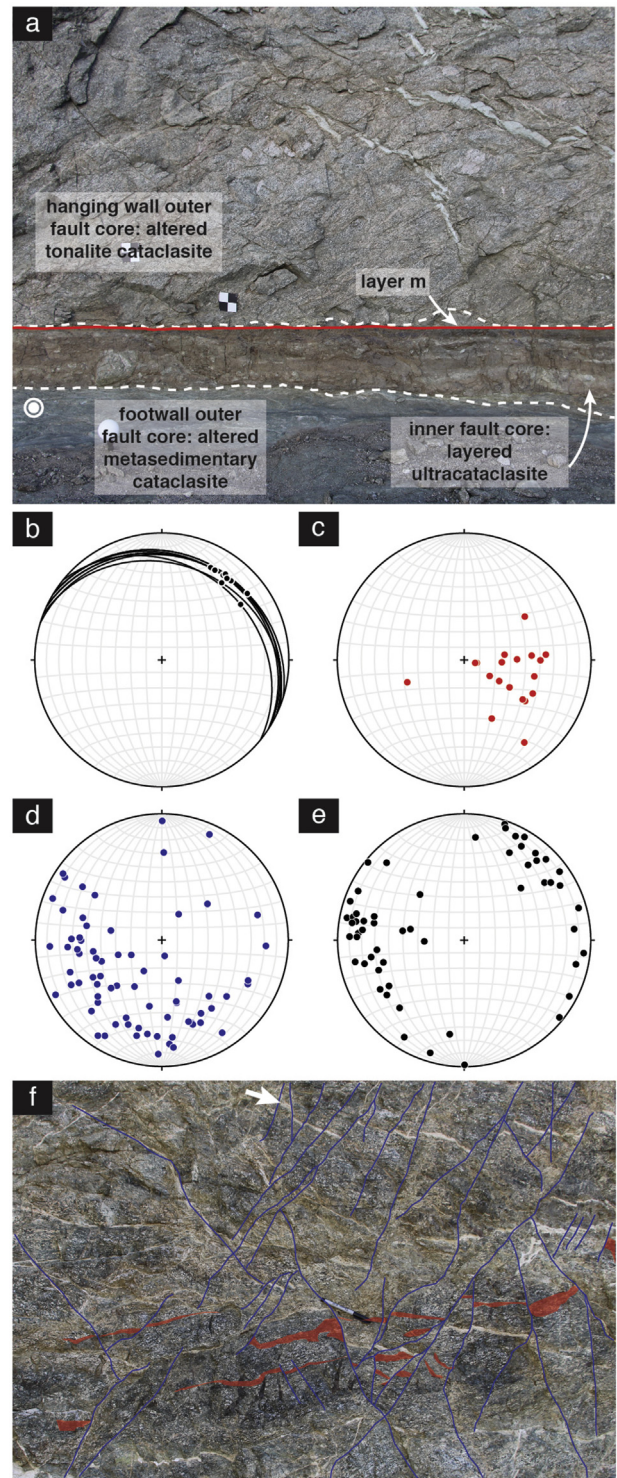
Fig. 3. Architecture of the La Quinta Fault: a: photograph illustrating the internal architecture of the La Quinta Fault. View is approximately in the down-dip direction to the NNE. Layer m is identified with the red line, the dashed white lines show the boundaries of the inner fault core, and the bull's-eye shows the slip sense in the viewing direction. b: fault orientation data measured at 14 locations along strike including the trend and plunge of slickenlines on exposed fault surfaces. c: Poles to pseudotachylite fault veins in the hangingwall damage zone. d: Poles to shear fractures within the hangingwall outer fault core. e: Poles to shear fractures in the hangingwall damage zone. f: Photograph showing hangingwall outer fault-core shear fractures (blue) with normal-sense apparent offsets. White arrow indicates a thin dyke that is offset and example pseudotachylite fault veins that are offset in red. View to the SE, approximately orthogonal to dip on the La Quinta Fault. (For interpretation of the references to colour in this figure legend, the reader is referred to the web version of this article.)
