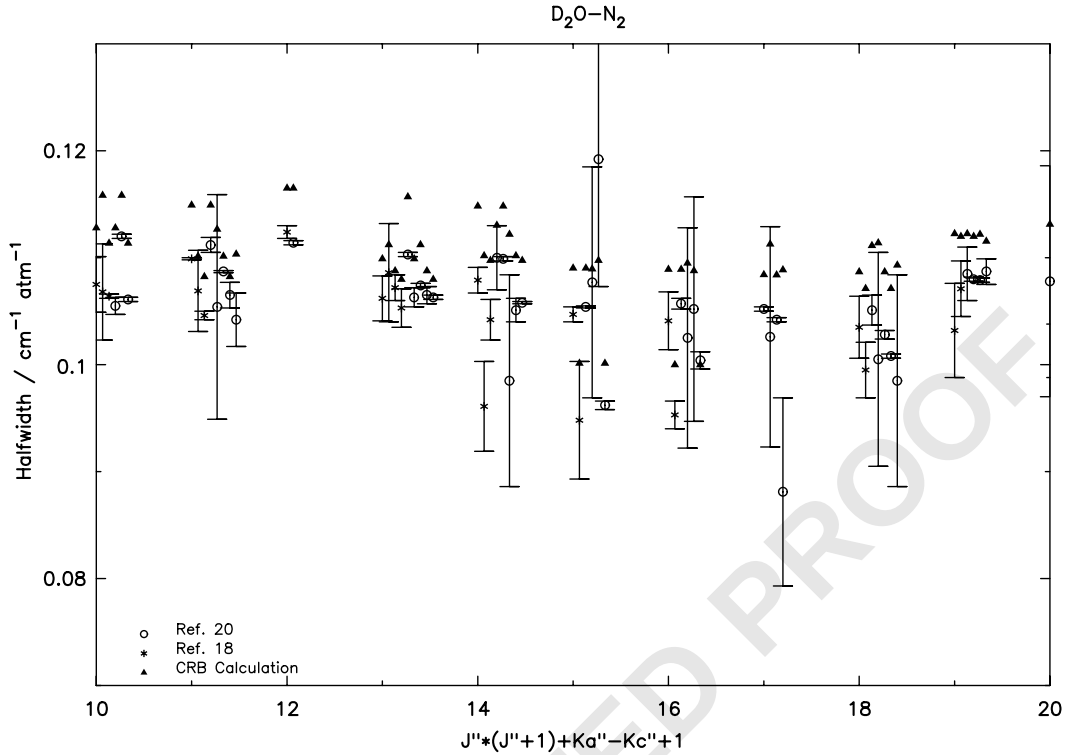
Fig. 4. Measured [18,20] and CRB calculated half-widths for the D_2O-N_2 system versus an energy-ordered index, J''*(J''+1)+Ka''-Kc''+1 . The range of the x -axis was chosen to demonstrate the comparison of the data.
