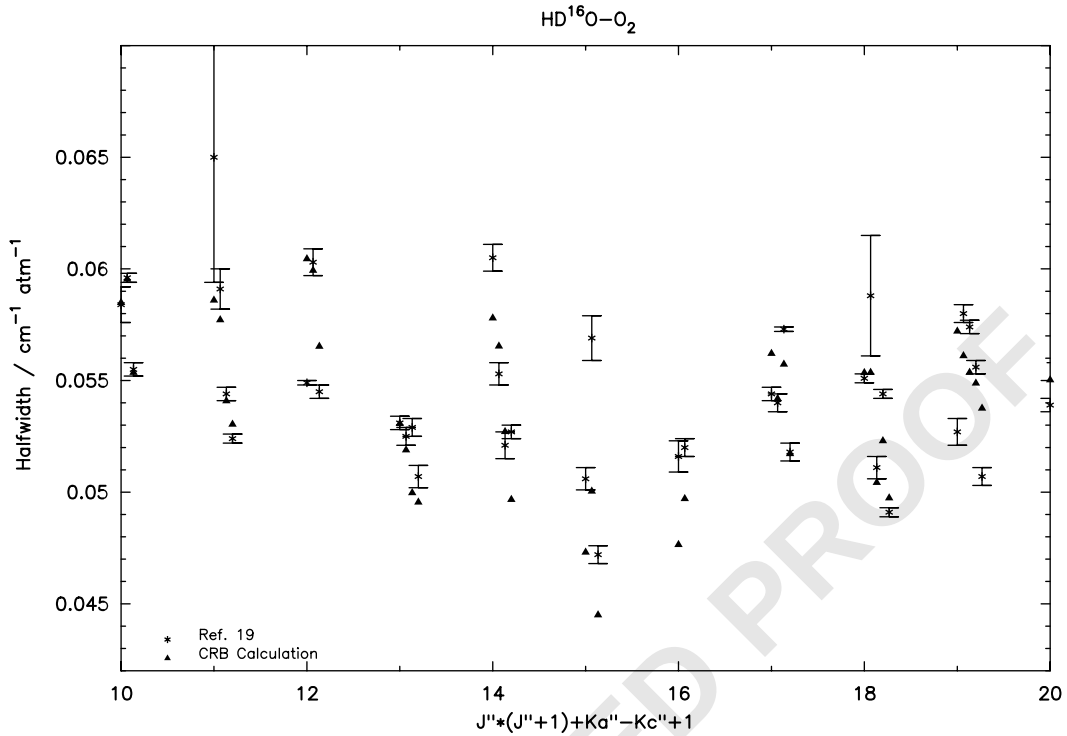
Fig. 5. Measured [19] and CRB calculated half-widths for the HDO-O 2 system versus an energy-ordered index, J^*(J+1)+K_a-K_c+1 . The range of the x-axis was chosen to demonstrate the comparison of the data.
