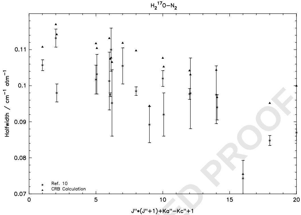
Fig. 2. Measured [10] and CRB calculated half-widths for the \text{H}_2^{17}\text{O}-\text{N}_2 system versus an energy-ordered index, J^*(J+1)+K_a-K_c+1 . The range of the x -axis was chosen to demonstrate the comparison of the data.
