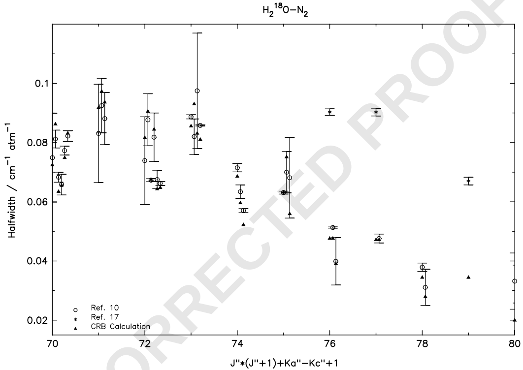
Fig. 1. Measured [10,17] and CRB calculated half-widths for the H 2 18 O-N 2 system versus an energy-ordered index, J''*(J''+1)+Ka''-Kc''+1 . The range of the x-axis was chosen to demonstrate the comparison of the data.
