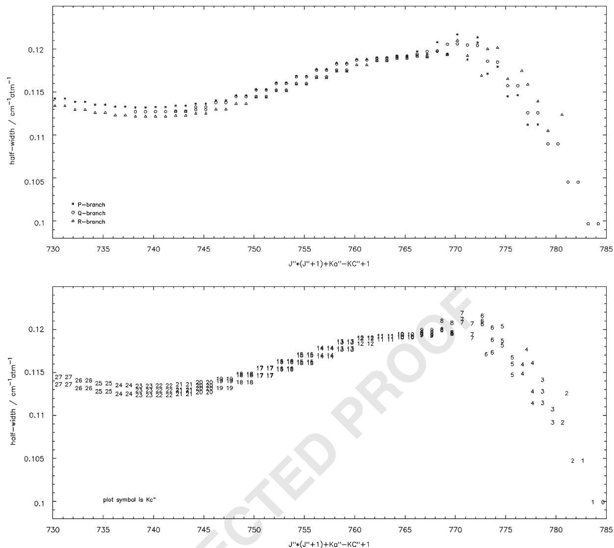
Fig. 2. Top panel: Calculated N_2 -broadened half-widths at 296 K for transitions with J'' = 27 versus the rotational state index, (J''*(J''+1)+K\alpha''-Kc''+1) , plotted are the data for index running from 730 ( 27_{027} ) to 784 ( 27_{270} ). The symbols are an asterisk (*) for the P-branch, open circle (○) for the Q-branch, and open delta ( \Delta ) for the R-branch transitions. Bottom panel: Same as above with plot symbols equal to Kc'' .
