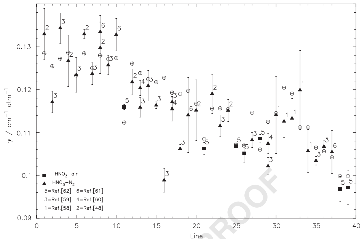
Fig. 6. \text{N}_2 -broadened (solid triangle symbols, ▲) and air-broadened (solid square symbols, ■) measurements with 2-sigma error bars, and the CRB calculated ( \text{N}_2 -broadened or scaled to air by 0.936) values (⊕ symbols) versus the line count. Half-widths are in units of \text{cm}^{-1} \text{atm}^{-1} at 296 K.
