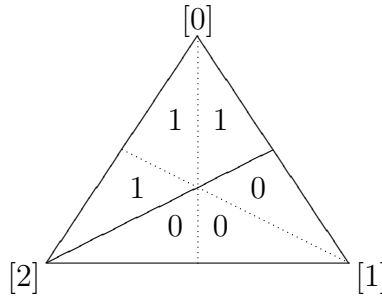
FIG. 1. The partitioning of \text{Sd}^1 \Delta_2 . Triangles belonging to H_i are marked i .
