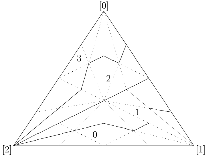
FIG. 2. The partitioning of \text{Sd}^2 \Delta_2 . Only one triangle in each region H_i is marked i .
