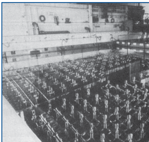
Spent Fuel in Pool Storage at a Nuclear Power Plant
