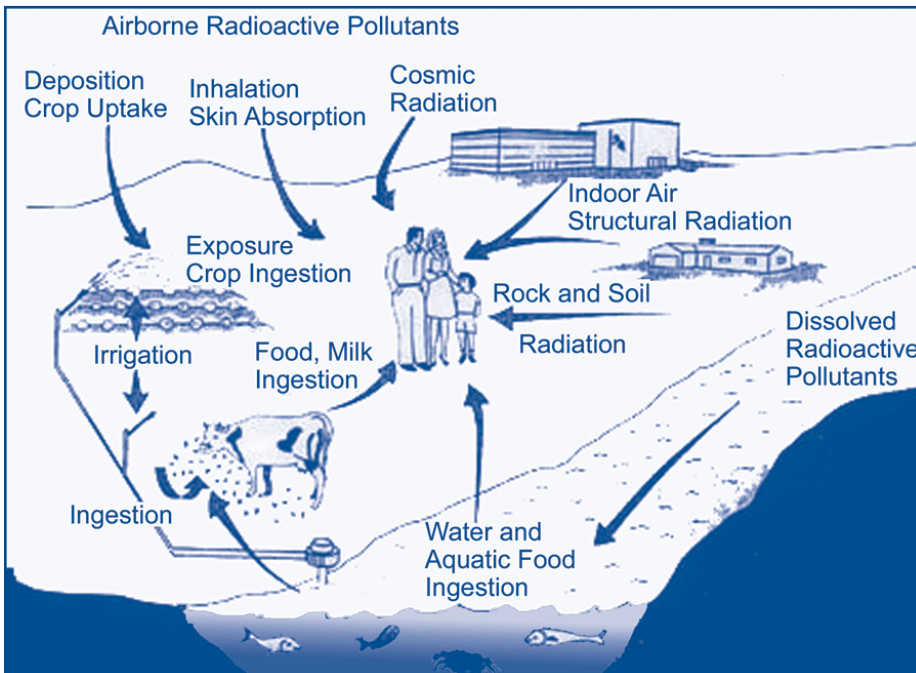
Figure 31. Major Pathways by Which Dispersed Radionuclides Can Affect Living Organisms
