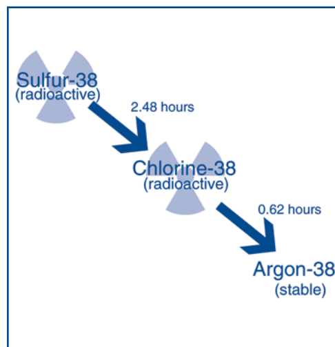
Figure 3. Radioactive Decay
