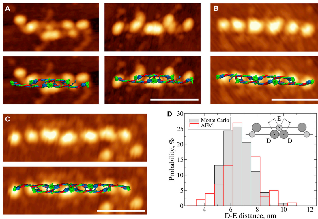
Figure 4. AFM Images and In Silico Structures of Two-Stranded Fibrin Oligomers
