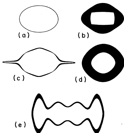
FIG. 1. (a) Elliptical orbit for an oscillator described by Eqs. (12). The abscissa is q , the ordinate is p . The major-to-minor axis ratio of unity has been increased in plotting to fit the Tektronix hard-copy screen area symmetrically. This same increase applies to each figure. All data were obtained on the Digital Equipment Corporation VAX 11/780 computer at the Physics Department (Lausanne) using a fourth-order Runge-Kutta integration in double precision with time steps in the range 0.01 down to 0.001. (b) Long-time qp trajectory for Eqs. (13) or (14) with initial values q=1 , p=1 , s=1 , p_s=0 , and Q=1 . (c) Same as (b) with Q=0.1 . (d) Long-time qp trajectory for Eqs. (15) with initial values q=1 , p=1 , \xi=0 , and Q=1 . (e) Same as (d) with Q=0.1 .
