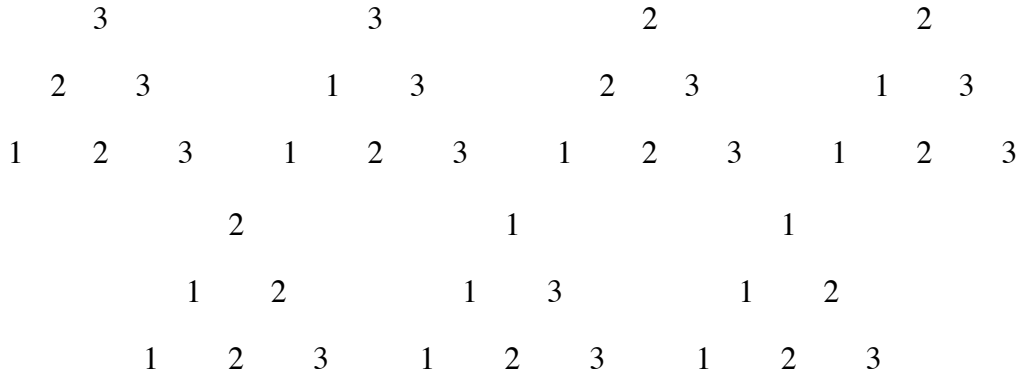
Figure 7: The seven monotone triangles of order 3.
