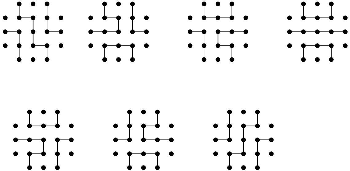
Figure 14: The seven FPL states of order 3.
