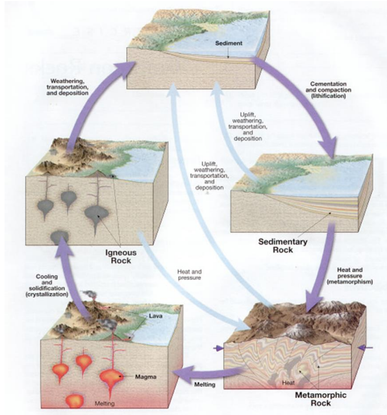
Figure 1. The rock cycle illustrates the role of various geologic processes in the formation of rocks. From Tarbuck, Lutgens, and Pinzke (2003).
