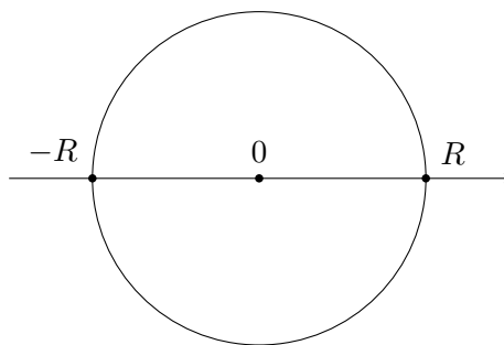
FIGURE 1. Radius of convergence
