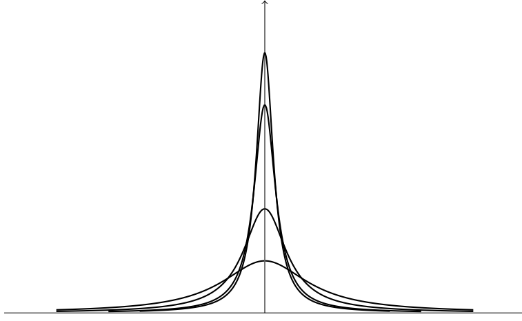
FIGURE 6. Approximation of unity
