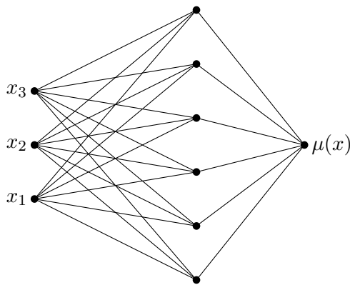
FIGURE 7. Visualization of \mu when n = 3 and m = 6 .
