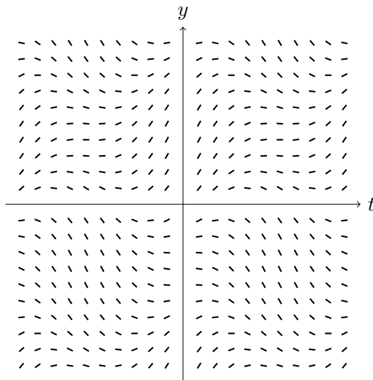
FIGURE 8. Visualization of F(t, y) .
