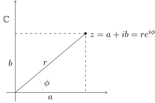
FIGURE 2. Polar and cartesian coordinates in the complex plane
