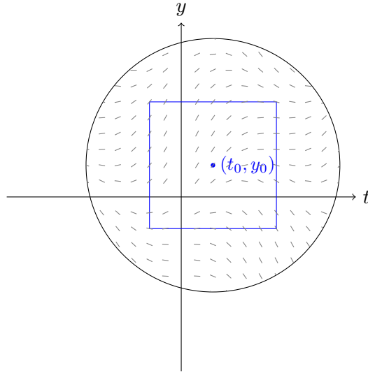
FIGURE 9. Visualization of F(t, y) .
