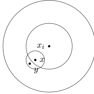
FIGURE 3. The balls B_{x_i} , B(x_i, \delta_{x_i}) , B(x, \delta) .
