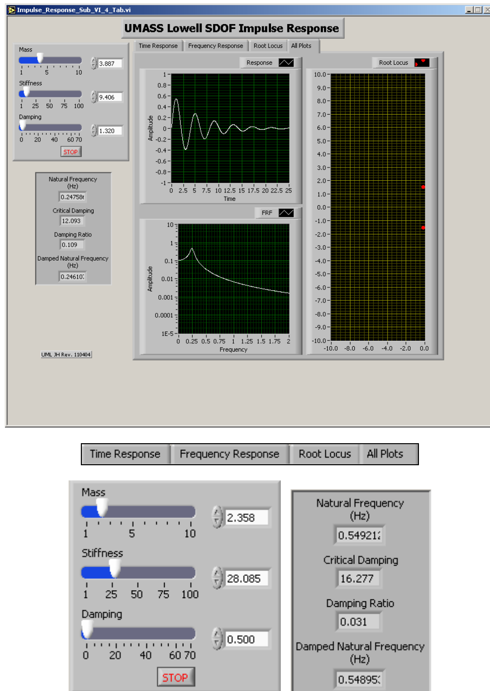
Figure 5 – LabVIEW 2 nd Order System Characterization
