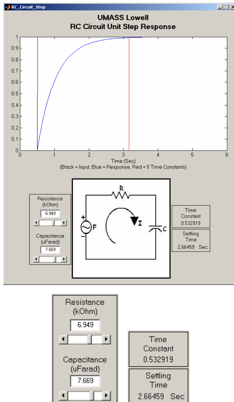
Figure 1 – MATLAB 1 st Order System Characterization – Time Response
